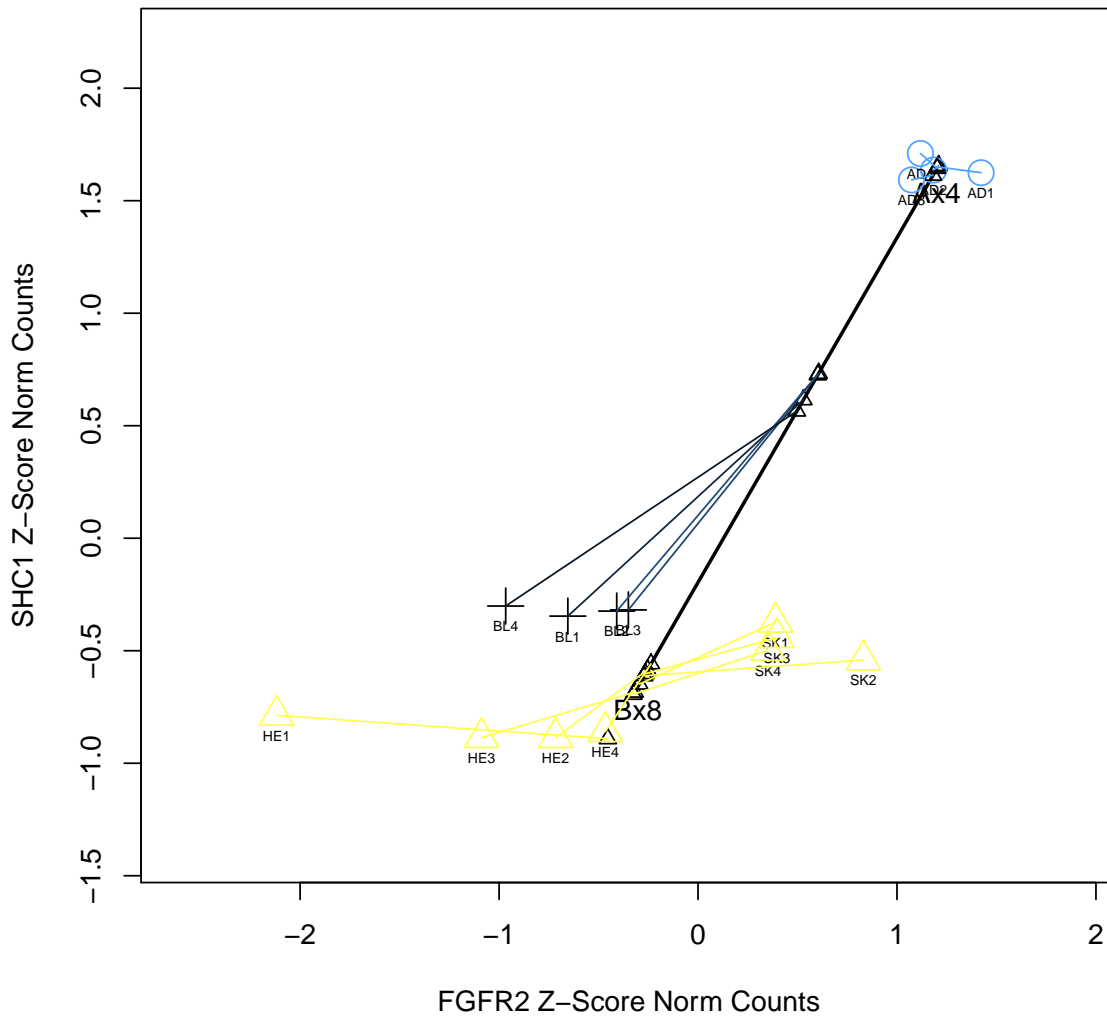
Figure 6: OUT\SCGO\GSEPD.Ax4.Bx8.GO0004713.pdf First page of the projections file for one GO Term. All significant sets have this figure generated displaying the central axis between two groups as a black line (with ends annotated Ax4 and Bx8), and each sample's closest point along the line. These files have half as many pages as genes in the set, so we can display pairs as two-dimensional scatterplots. It's a workaround to the problem of displaying an N-dimensional scatterplot. For sets with fewer than 11 genes, full pairings are viewable with the Pairs file, Figure 7
