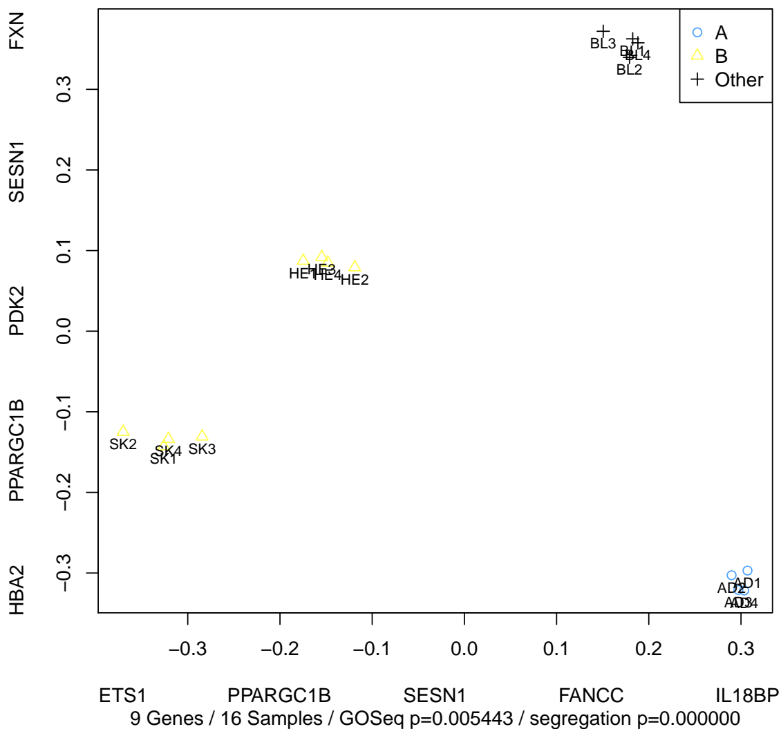
Figure 8: OUT\SCGO\Scatter.Ax4.Bx8.GO0000302.pdf The Scatter file is similar to the PCA files, but the gene set is restricted to those within a given, significant, GO Term. As in the PCA file, genes driving the principle components are annotated along the axes. At the bottom of the figure, statistics are given pertaining to this group. All such data is available in tables, but this Scatter plot helps the user see which samples behave like which groups. Depending on the number of genes relative to the number of samples, different PCA formulas may be used. For a set with only two genes, this file can directly display the expression values as normalized counts, the same as found on the expression heatmap (Fig. 5.)
