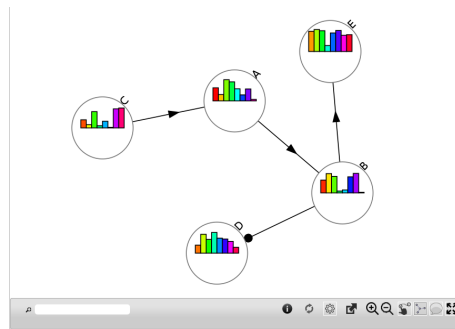
Figure 8: Barplots inside nodes
